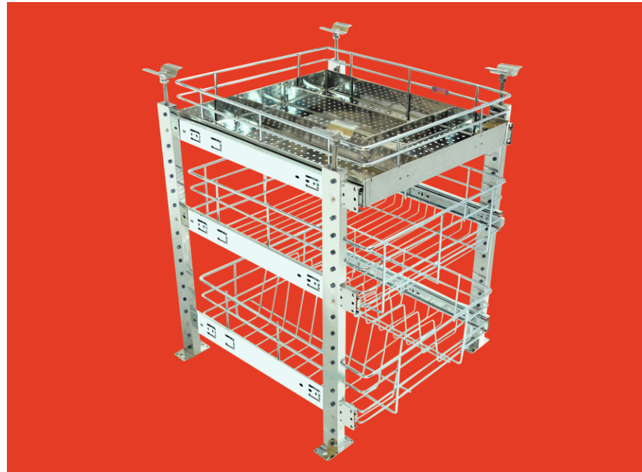
★ CORNER (Double) Dimensions 9"x9" | H-17"
